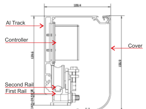
Cross Section of Aluminum Track
